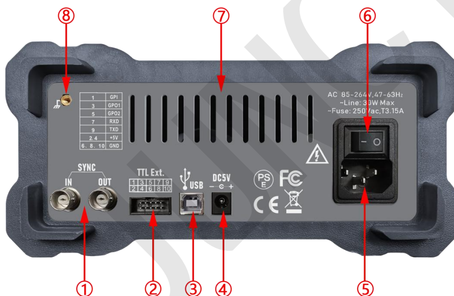
Figure 2-2-1 PSG9000 rear panel
