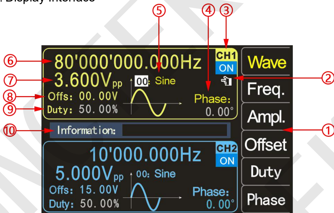
Figure 2-3-1 PSG9000 display interface
