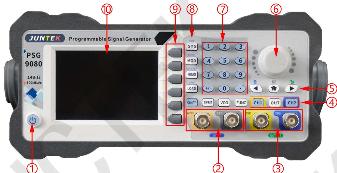
Figure 2-1-1 PSG9000 front panel
